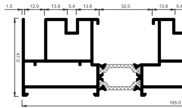
Three rail
