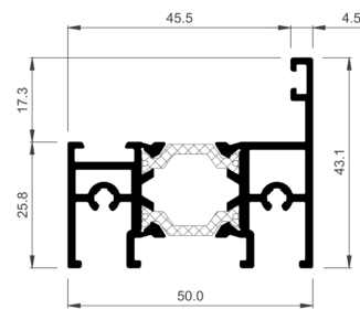
Central sash
