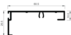
Fixed sash frame cover
