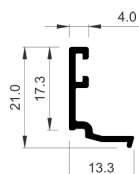
Glazing bead 4mm Triple glazed
