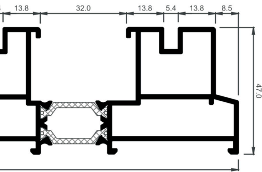
frame
