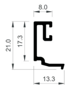
Glazing bead 8mm Double glazed
