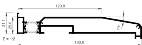
Cill 180mm
