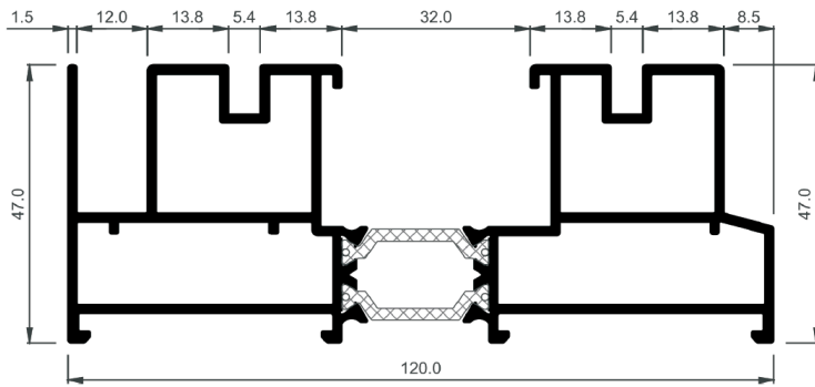
Two rail frame
