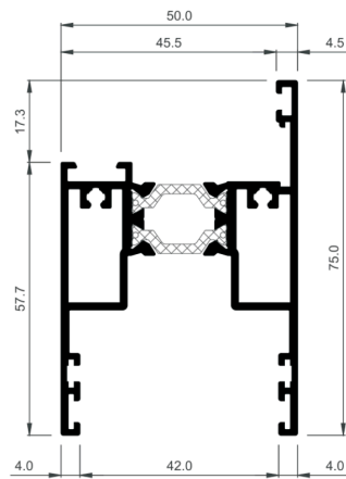
Perimeter sash
