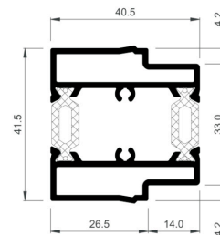
Sash joint profile
