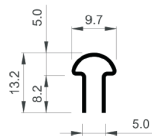
Stainless steel rail
