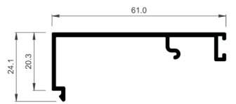
Frame cover for fixed light
