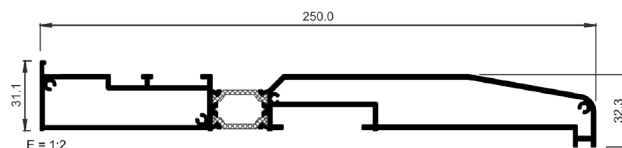
Cill 250mm
