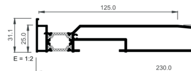
Cill 230mm
